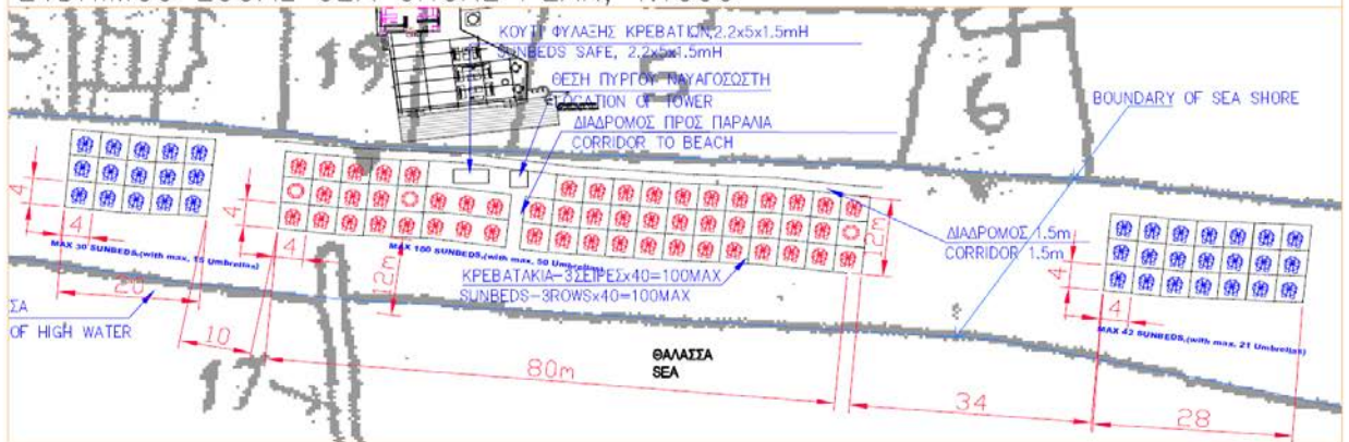
EVDHIMOU LOCAL SEA SHORE PLAN, 1:1000
